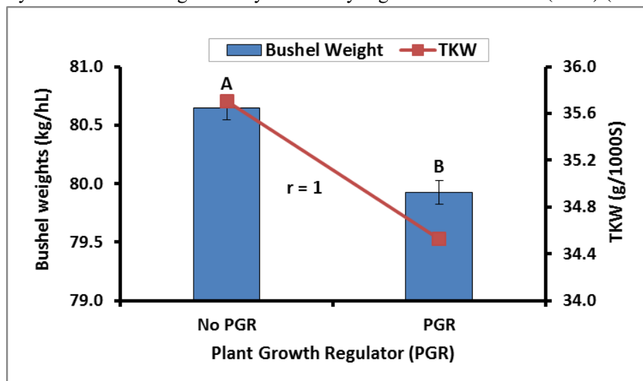
Figure 3: Relationship between bushel weight ( columns ) (kg/hL) and TKW ( line ) (g/1000s) with the application of PGR for the 2015 growing season at Scott, SK. Vertical bars followed by the same letters are not significantly different according to Tukey’s Honestly Significant Difference (HSD) ( P > 0.05 ).
