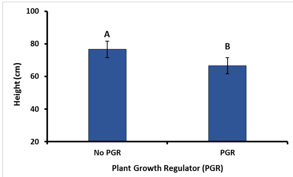
Figure 1: Effects of PGR on plant height (cm) in wheat for the 2015 growing season at Scott, SK. Vertical bars followed by the same letters are not significantly different according to Tukey’s Honestly Significant Difference (HSD) ( P > 0.05 ).
