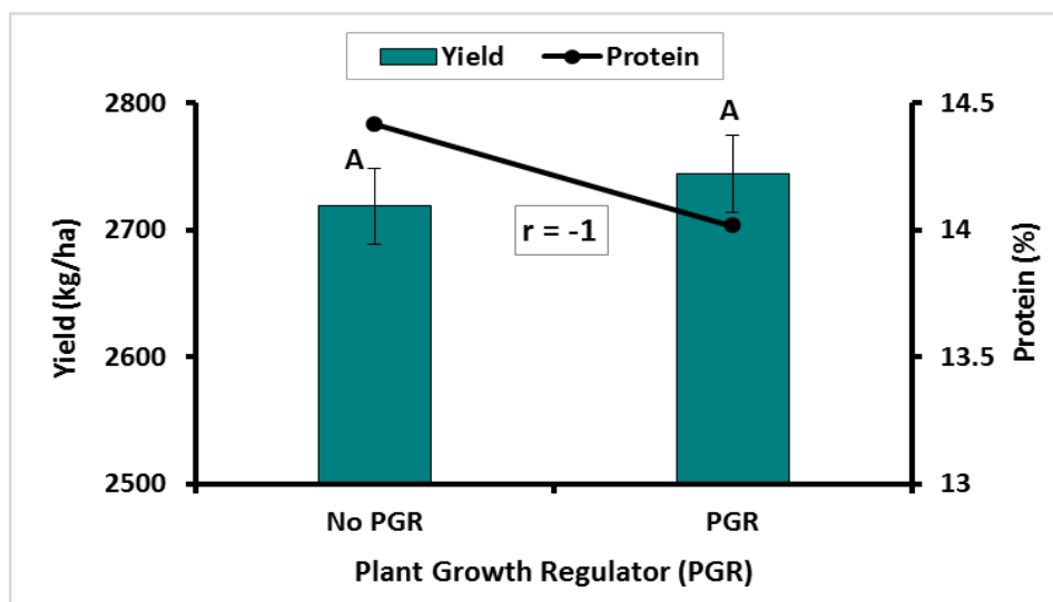
Figure 2: Relationship between wheat grain yield ( columns ) (kg/ha) and protein( line ) (%) with the application of PGR for the 2015 growing season at Scott, SK. Vertical bars followed by the same letters are not significantly different according to Tukey’s Honestly Significant Difference (HSD) ( P > 0.05 ).
